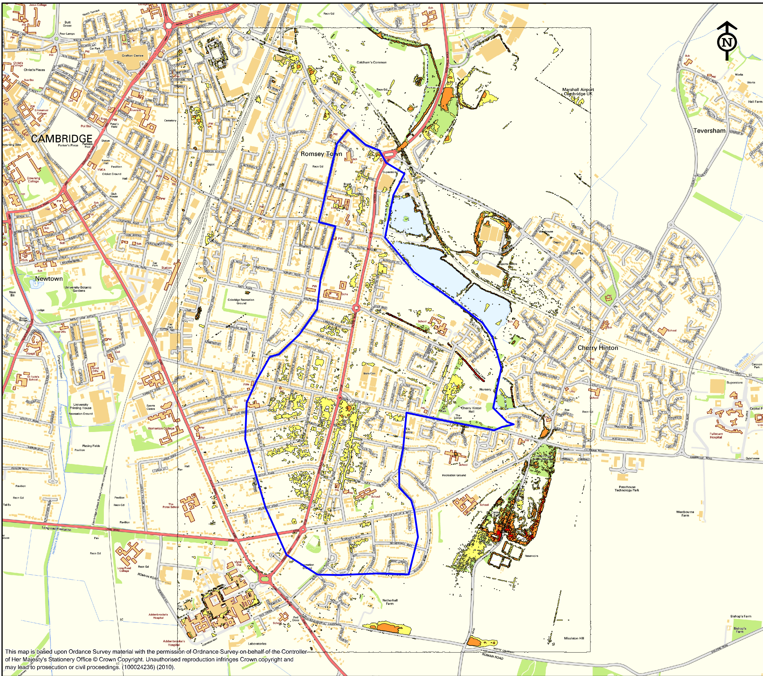
FIGURE G6 0.5% AEP "DO SOMETHING" PLUVIAL MODELLING MAXIMUM HAZARD - CHERRY HINTON
